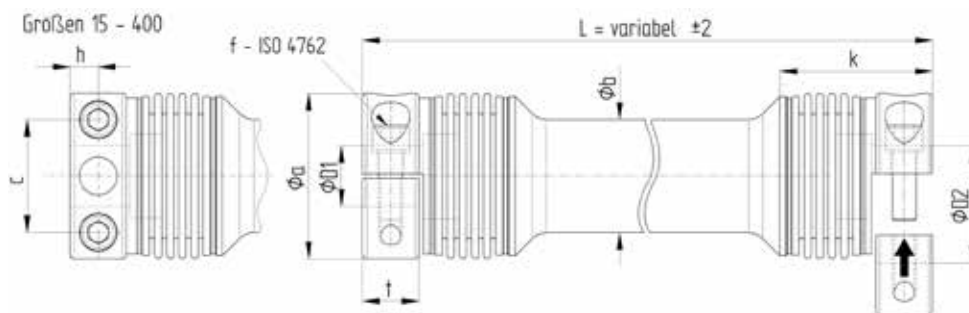
metal bellows coupling EWV
