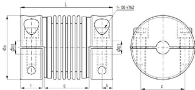
metal bellows couplings EWMH
